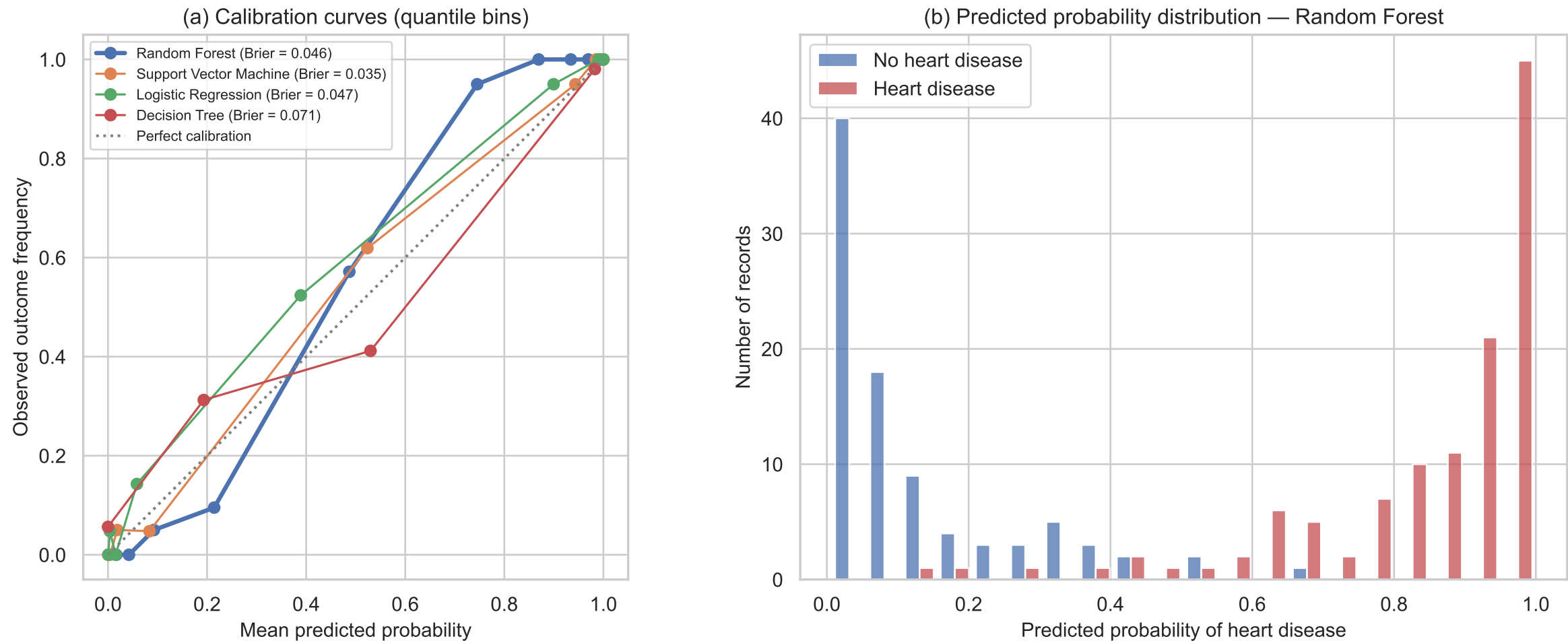
Figure 7. Calibration of predicted probabilities on the held-out test partition
